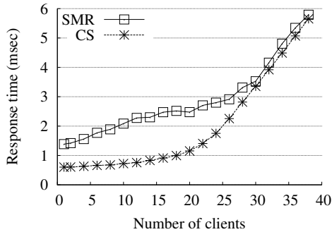
Figure 2. Client-server (CS) versus state-machine replication with one replica (SMR) executing read-only commands.
