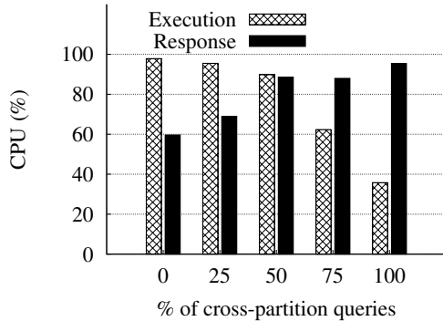
Figure 11. CPU utilization for the experiments in Figure 10.
