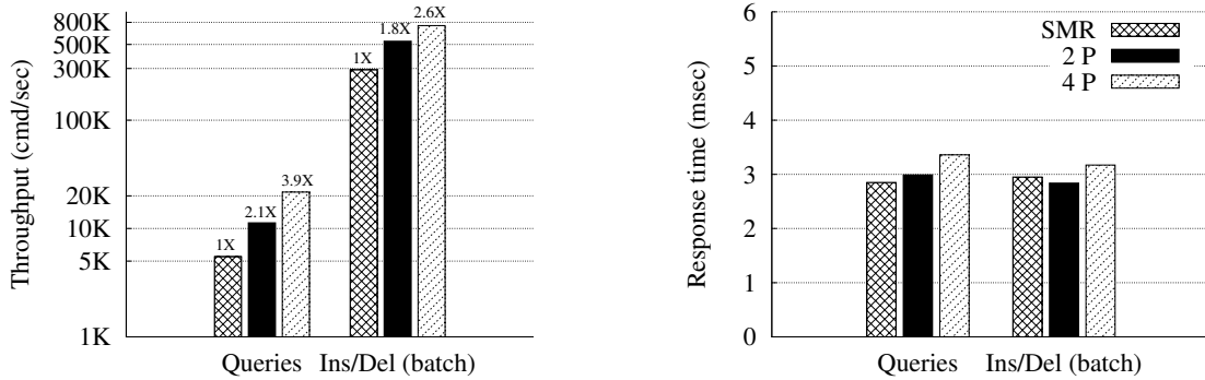
Figure 9. State partitioning (2 and 4 partitions) versus state-machine replication for queries and batched updates with no cross-partition commands. (Left) Throughput (y-axis in log scale) with improvement over SMR versus command type. (Right) Response time versus command type.
