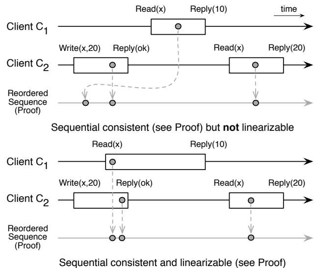
Figure 1. Linearizability vs. sequential consistency.
