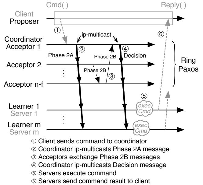
Figure 3. Ring Paxos in a client-server setup ( n acceptors, up to f of which can fail, and m learners/servers)
