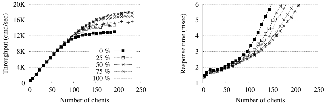
Figure 10. Effects of cross-partition queries in state partitioning. (Left) Throughput versus number of clients. (Right) Response time versus number of clients.
