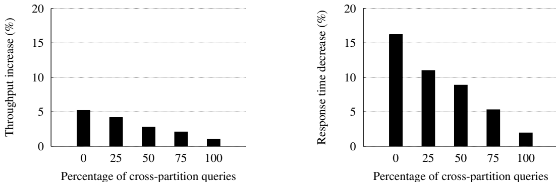
Figure 12. Improvements of speculative execution on state partitioning. (Left) Throughput increase versus percentage of cross-partition queries. (Right) Response time decrease versus percentage of cross-partition queries.
