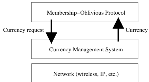
Figure 1. Membership-oblivious protocols
