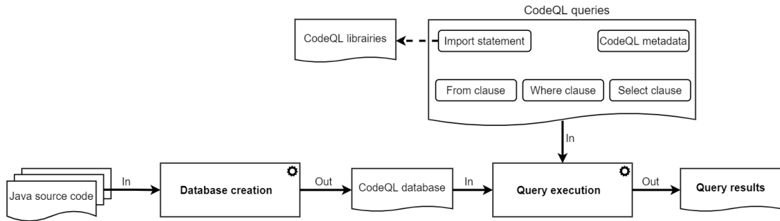
Figure 3.6: Representation of the CodeQL analysis process
