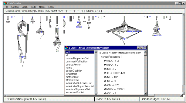
Figure 10. The CodeCrawler platform at work: (1) an inheritance tree with x node size = NIV, y node size = NOM, colour = NCV and (2) inspecting the data of a represented entity.
