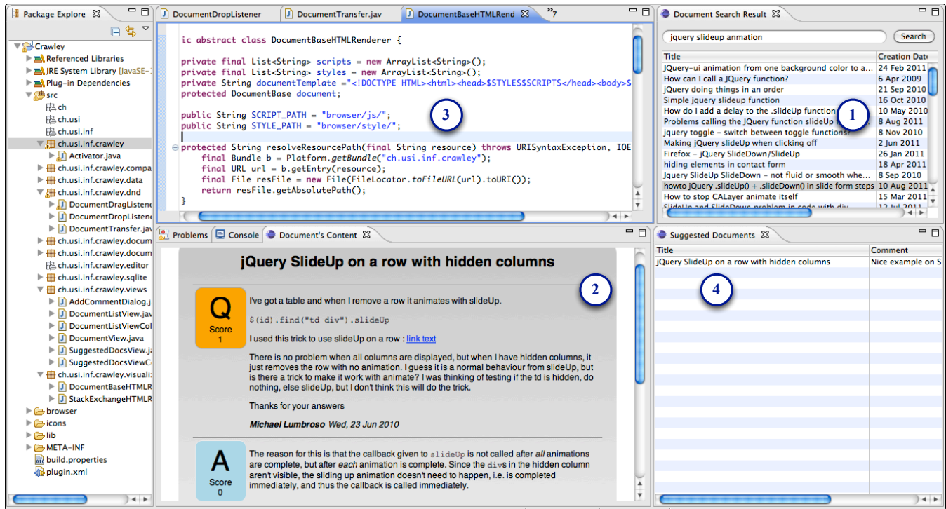
Figure 2. The Seahawk User Interface.
