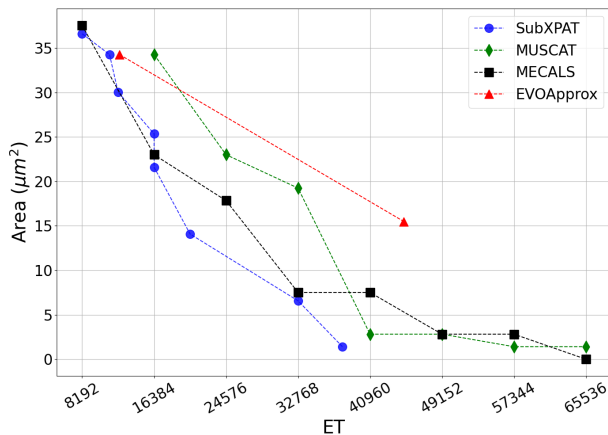
Fig. 12: Areas of approximations of a 16-bit adder.
