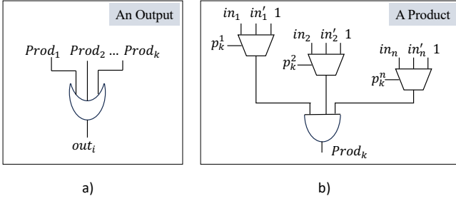
Fig. 1: Our 2-layer sum of products template. (a) A sum of K products. (b) A product of n primary inputs; parameter p_k^j determines how primary input in_j is to be handled.
