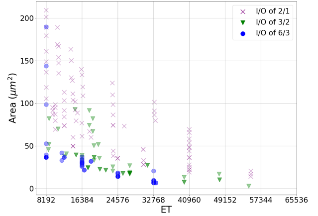
Fig. 10: Areas of SUBXPAT approximations of a 16-bit adder obtained with different I/O limits for subcircuit selection.
