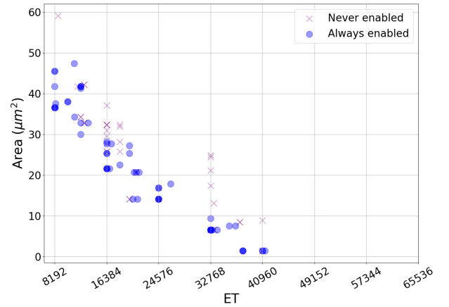
Fig. 11: Areas of SUBXPAT approximations of a 16-bit adder obtained with different constant resetting modes.
