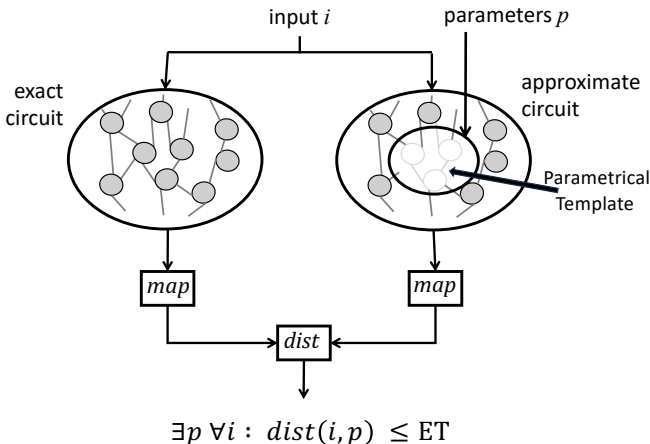
Fig. 4: Miter for SUBXPAT.
