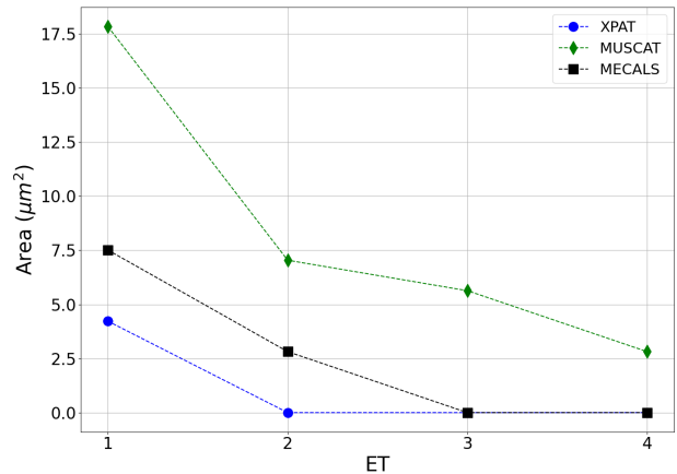
Fig. 8: Areas of approximations of a 2-bit adder.
