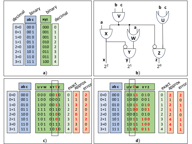
Fig. 7: Motivation for mnze_g calculation. (a) Truth table for an adder of 2 plus 1 bits (3 inputs and 3 outputs), in both binary and decimal. (b) A circuit implementing the truth table. (c) Perturbing the output of gate Y in a specific way (called here \hat{Y} ), makes the error at every truth table line be 2 or 0. Considering every possible perturbation, which can be done via the miter in Figure 6, makes the value of mnze_Y be derived to 2. (d) The effect of perturbing gate V propagates further through the circuit – a specific perturbation called \hat{V} is shown here, for which the error at every truth table line is 2, 1, or 0; the value of mnze_V , considering every possible perturbation, can be derived via the miter in Figure 6 to be 1.
