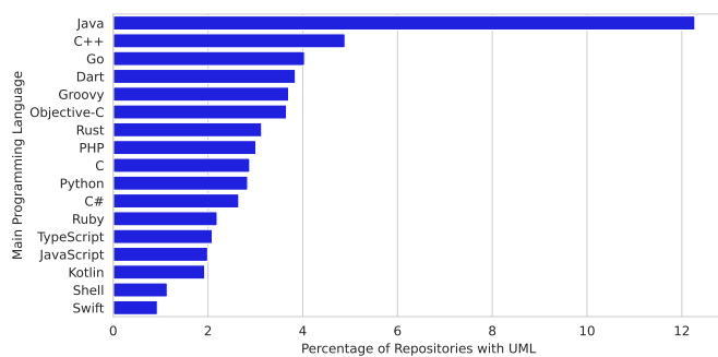
Fig. 4. Percentage of Repositories with UML by Language
