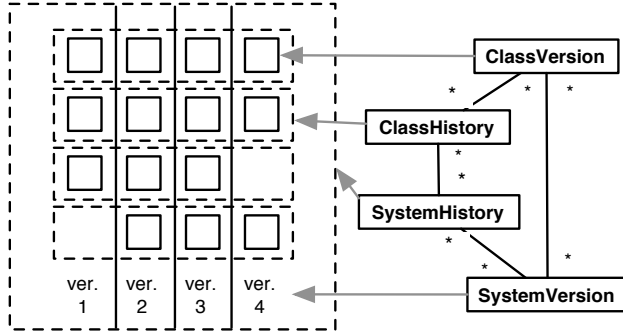
Figure 7. Example of building Hismo.
