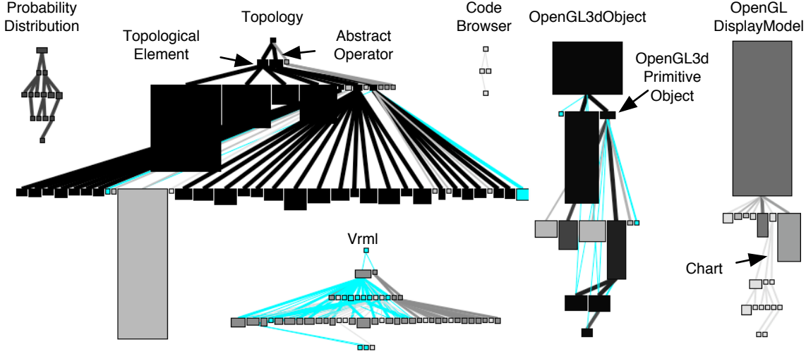
Figure 4. A Hierarchy Evolution Complexity View of the evolution of six hierarchies from the 40 versions of Jun.
