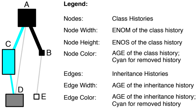
Figure 2. An example of the Hierarchy Evolution Complexity View.
