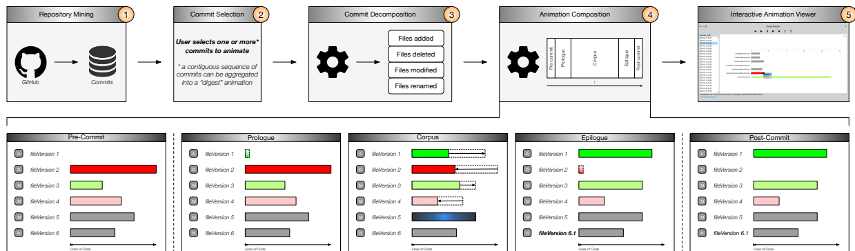
Fig. 1. Overview of the approach.
