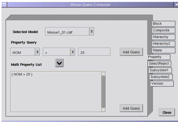
Figure 2. The Query Composition Window of MooseFinder.
