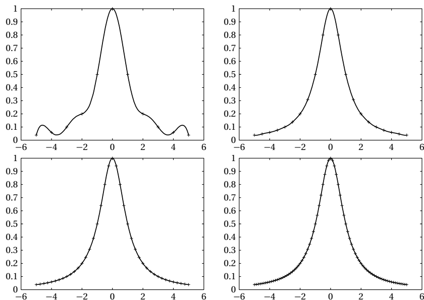
Figure 1: Interpolating Runge's example with d = 3 and n = 10, 20, 40, 80 .
