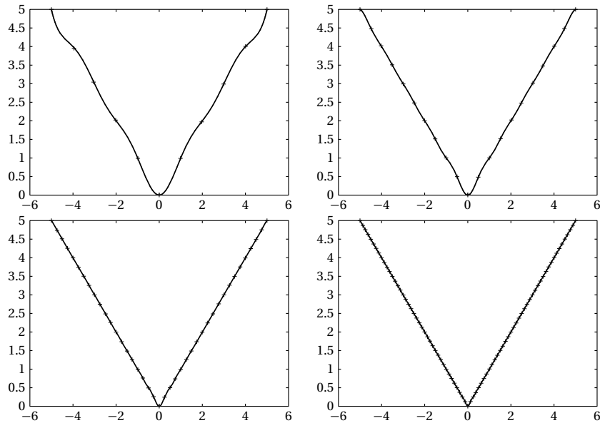
Figure 3: Interpolating |x| over [-5, 5] with d = 3 and n = 10, 20, 40, 80 .
