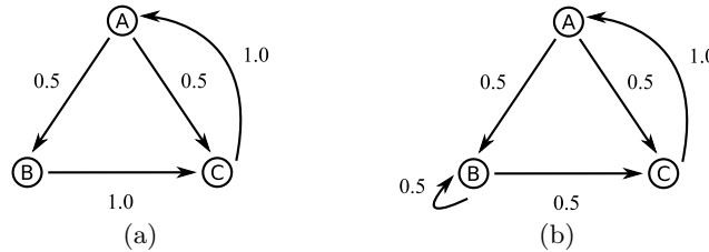
Fig. 1. An ergodic graph (a) Labeled with initial transition probabilities. (b) Balanced using a self-loop.
