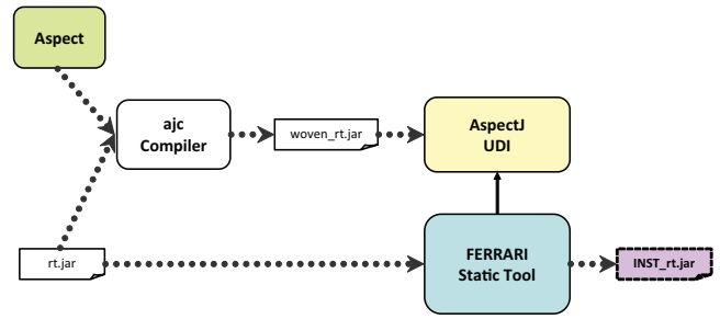
Figure 4: Static JDK instrumentation with the AspectJ UDI: First, ajc weaves the aspect into the JDK ( woven_rt.jar ). Afterwards, FERRARI inserts the bypasses in the woven JDK ( INST_rt.jar ).
