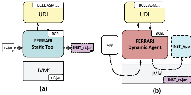
Figure 1: (a) Static and (b) dynamic instrumentation with FERRARI.
