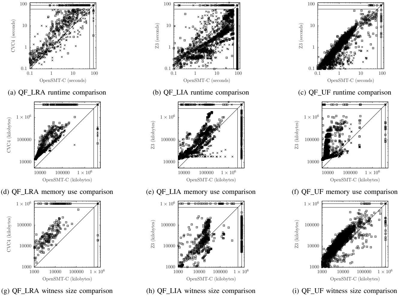
Fig. 3: Comparison between the two solvers with most witnesses produced, for each theory, both in witness producing mode; squares and crosses stand for UNSAT and SAT results, the top and right lines represent value limit, timeout, and memout.
