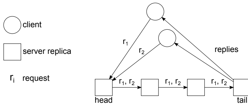
Figure 3.3. Chain replication.
