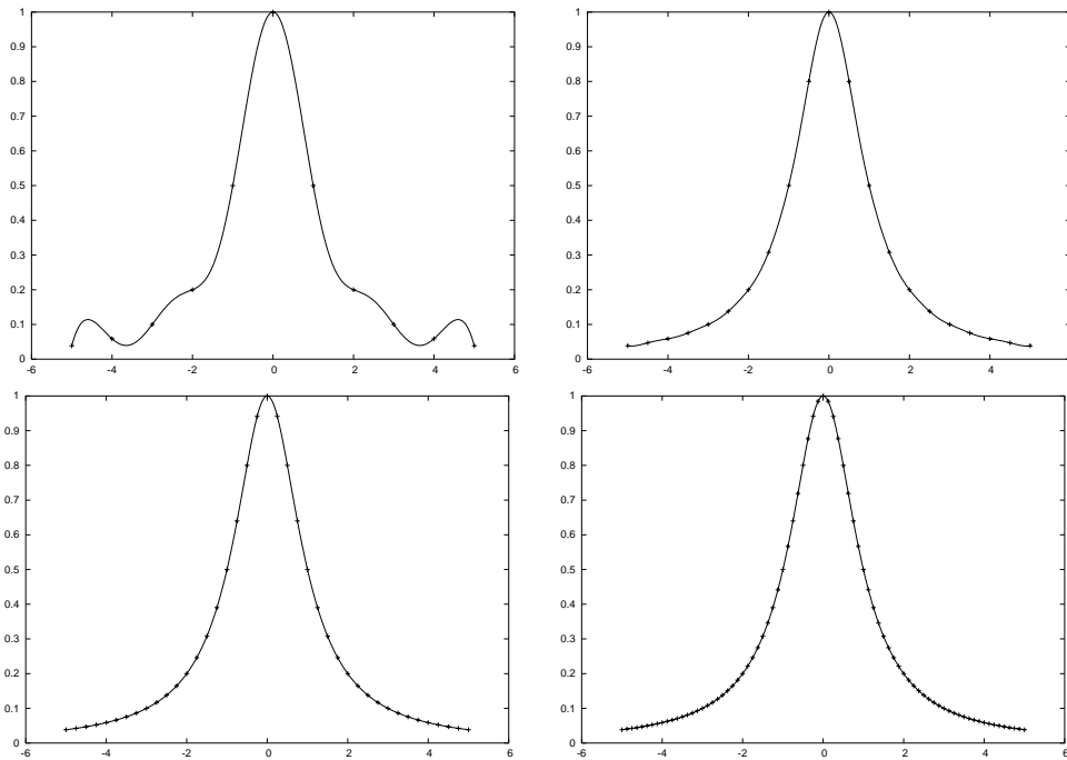
Figure 1: Interpolating Runge's example with d = 3 and n = 10, 20, 40, 80 .
