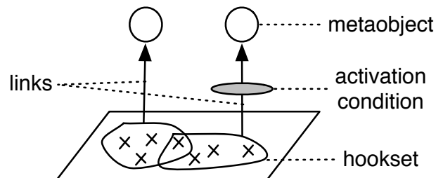
Figure 3: Hooksets, Links and Metaobjects in Geppetto
