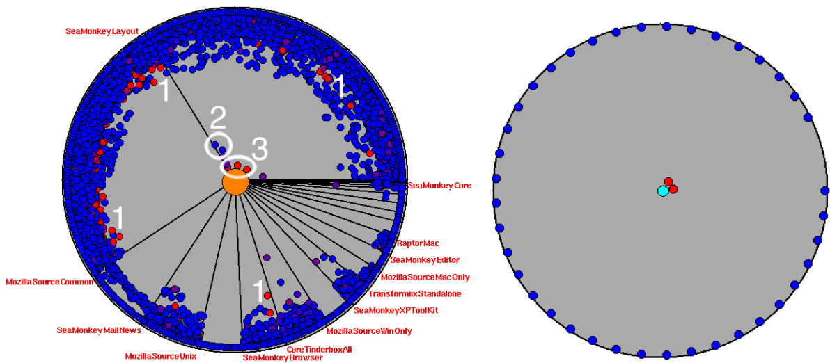
Figure 2: Evolution Radars for SeaMonkeyMailNews.
